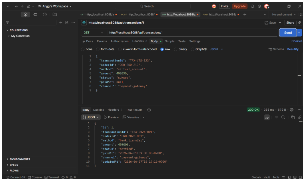
Gambar 3. 2 GET 2
