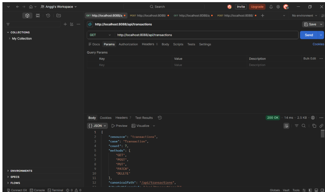
Gambar 3. 1 GET 1
