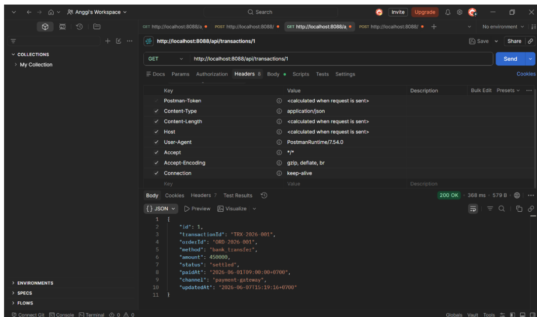
Gambar 3. 3 HEADER GET
