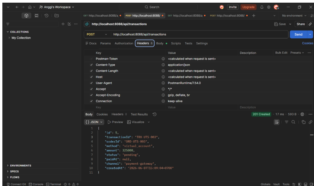
Gambar 3. 5 HEADER POST
