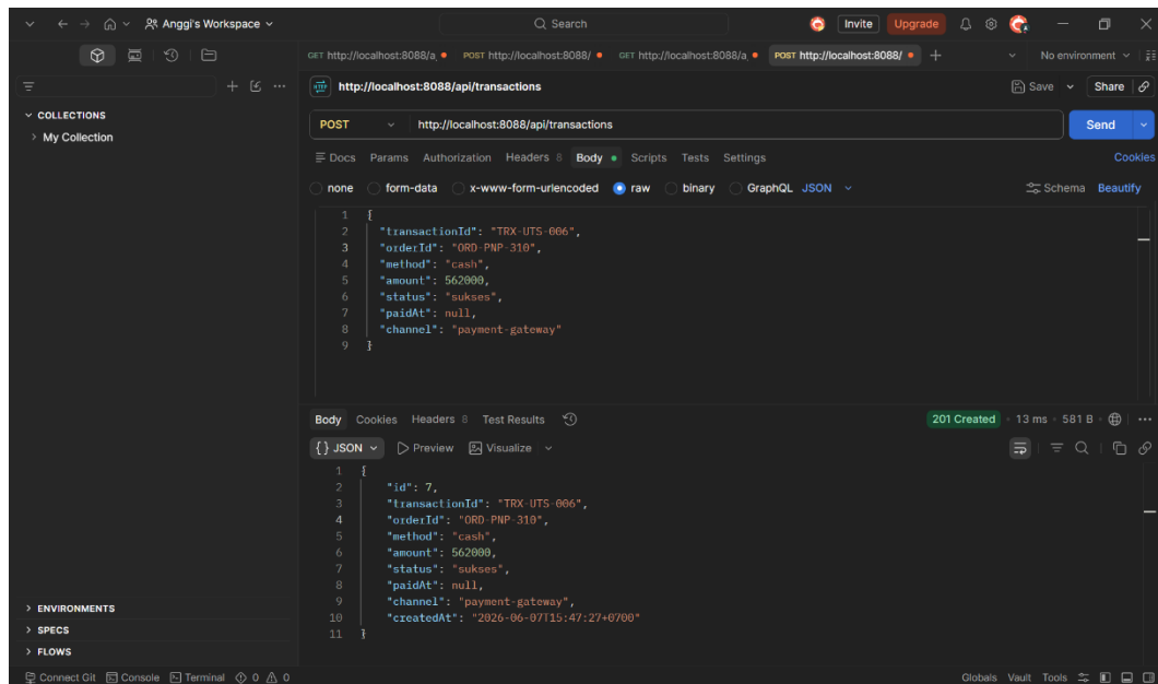
Gambar 3. 6 POST 2
