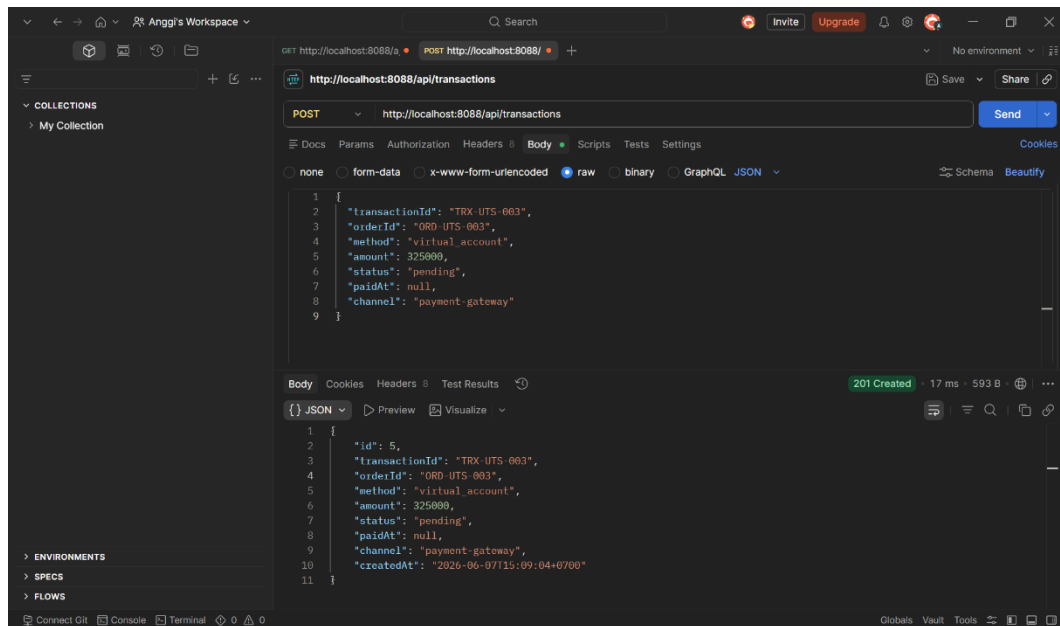
Gambar 3. 4 POST 1
